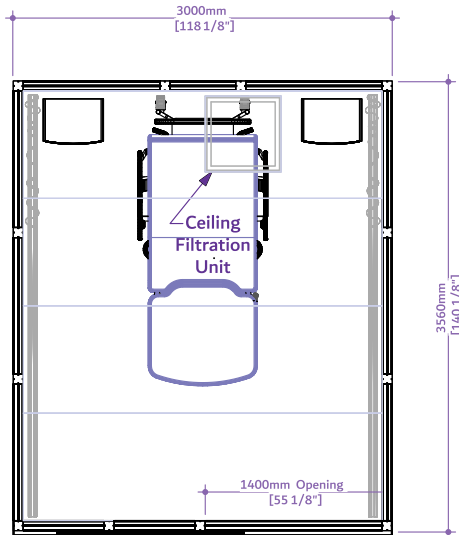
Sliding Door → Top View
