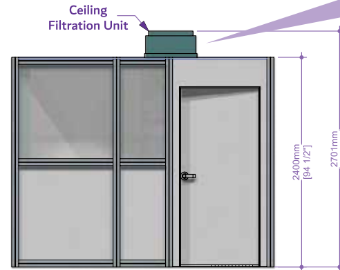
Front Elevation
